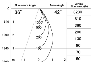
■ Direct Horizontal Illuminance SD287-0650B9030-DMWL
