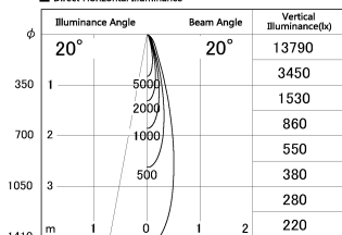
■ Direct Horizontal Illuminance SD287-0625B9035-DMWL
