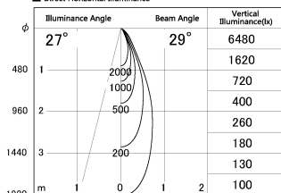
■ Direct Horizontal Illuminance SD287-0635B9035-DMWL
