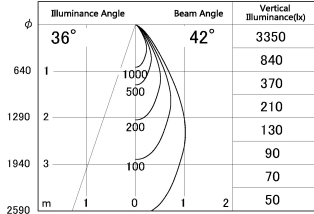
■ Direct Horizontal Illuminance SD287-0650B9035-DMWL
