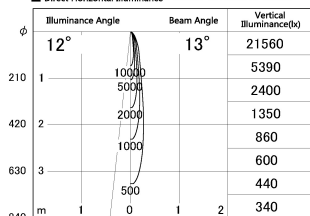
■ Direct Horizontal Illuminance SD287-0615B9040-DMWL
