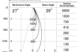
■ Direct Horizontal Illuminance SD287-0635B9040-DMWL
