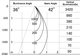
■ Direct Horizontal Illuminance SD287-0650B9040-DMWL
