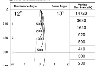
■ Direct Horizontal Illuminance SD287-0615WHC27-DMWL
