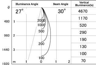
■ Direct Horizontal Illuminance SD287-0635WHC27-DMWL
