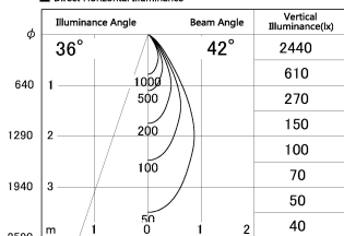
■ Direct Horizontal Illuminance SD287-0650WHC27-DMWL
