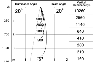
■ Direct Horizontal Illuminance SD287-0625WHC30-DMWL
