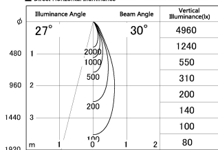
■ Direct Horizontal Illuminance SD287-0635WHC30-DMWL
