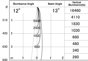
■ Direct Horizontal Illuminance SD287-0615WHC35-DMWL
