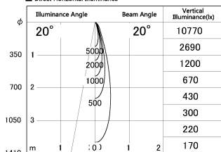
■ Direct Horizontal Illuminance SD287-0625WHC35-DMWL
