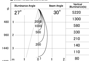
■ Direct Horizontal Illuminance SD287-0635WHC35-DMWL
