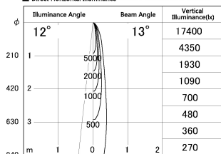
■ Direct Horizontal Illuminance SD287-0615WHC40-DMWL
