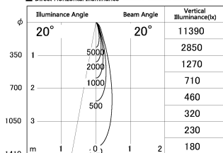
■ Direct Horizontal Illuminance SD287-0625WHC40-DMWL
