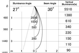
■ Direct Horizontal Illuminance SD287-0635WHC40-DMWL
