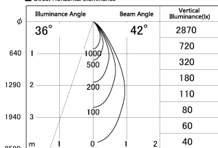
■ Direct Horizontal Illuminance SD287-0650WHC40-DMWL
