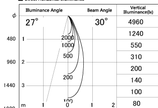
■ Direct Horizontal Illuminance SD287-0635BHC30-DMWL
