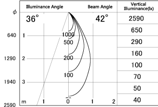
■ Direct Horizontal Illuminance SD287-0650BHC30-DMWL
