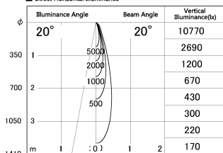
■ Direct Horizontal Illuminance SD287-0625BHC35-DMWL
