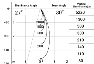
■ Direct Horizontal Illuminance SD287-0635BHC35-DMWL
