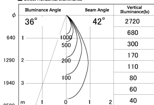
■ Direct Horizontal Illuminance SD287-0650BHC35-DMWL
