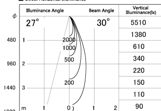
■ Direct Horizontal Illuminance SD287-0635BHC40-DMWL
