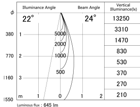
■ Direct Horizontal Illuminance SD374-1125B9027-IK
