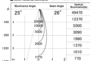
■ Direct Horizontal Illuminance SD376-3725B9027-LX
