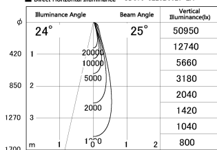
■ Direct Horizontal Illuminance SD376-3225B9027-LX
