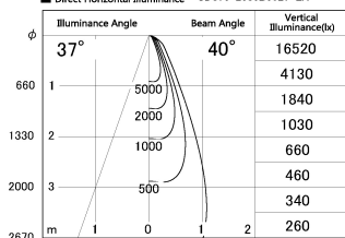
■ Direct Horizontal Illuminance SD376-2535B9027-LX
