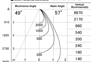
■ Direct Horizontal Illuminance SD376-2555B9027-LX
