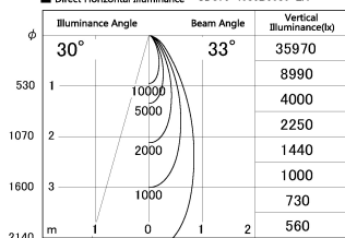
■ Direct Horizontal Illuminance SD376-4035B9030-LX
