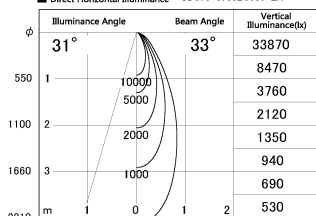
■ Direct Horizontal Illuminance SD376-3735B9030-LX
