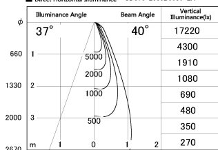
■ Direct Horizontal Illuminance SD376-2535B9030-LX
