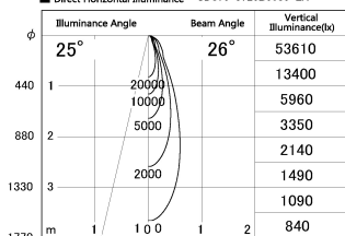
■ Direct Horizontal Illuminance SD376-3725B9035-LX
