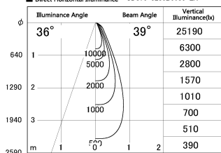
■ Direct Horizontal Illuminance SD376-3235B9035-LX
