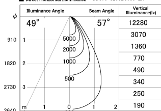
■ Direct Horizontal Illuminance SD376-3255B9035-LX
