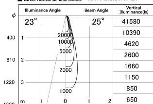
■ Direct Horizontal Illuminance SD376-2525B9035-LX
