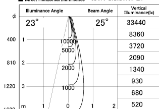
■ Direct Horizontal Illuminance SD376-2025B9035-LX
