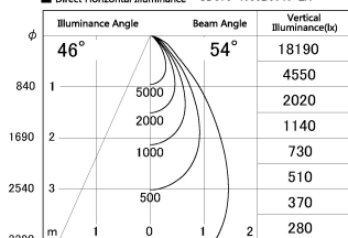
■ Direct Horizontal Illuminance SD376-4055B9040-LX
