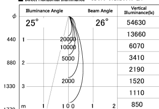
■ Direct Horizontal Illuminance SD376-3725B9040-LX
