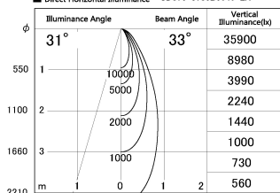
■ Direct Horizontal Illuminance SD376-3735B9040-LX
