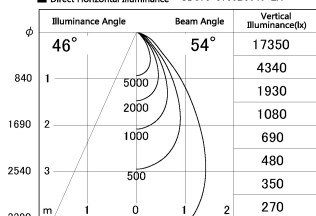
■ Direct Horizontal Illuminance SD376-3755B9040-LX
