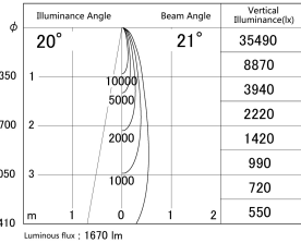
■ Direct Horizontal Illuminance SD379-1520W9027
