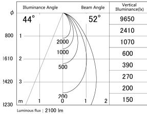
■ Direct Horizontal Illuminance SD379-2050W9035
