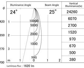
■ Direct Horizontal Illuminance SD379-1525W9040
