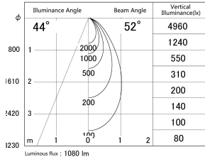
■ Direct Horizontal Illuminance SD379-1050B9027S
