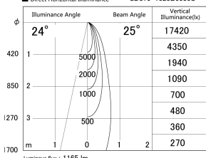
■ Direct Horizontal Illuminance SD379-1025B9030S
