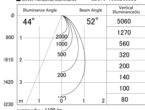
■ Direct Horizontal Illuminance SD379-1050B9030S
