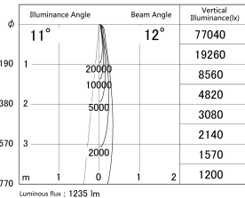
■ Direct Horizontal Illuminance SD379-1610W9027-IK
