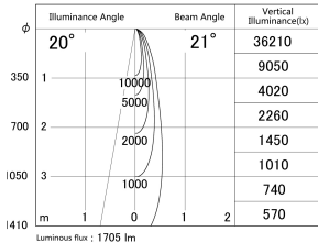
■ Direct Horizontal Illuminance SD379-1520W9030S-IK
